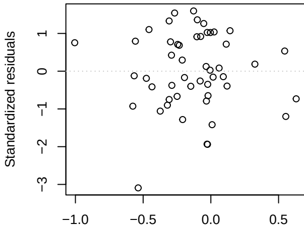
Standardized Residuals vs Fitted
