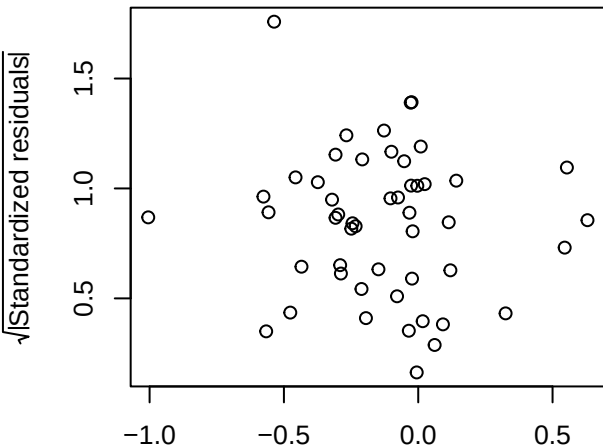
Scale-Location
